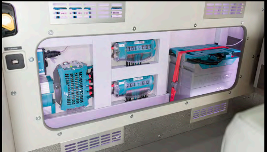
Mastervolt® power supply with a lithium-ion battery, Mass Combi (charger and inverter in the same housing), charge booster and Masterbus control units.
